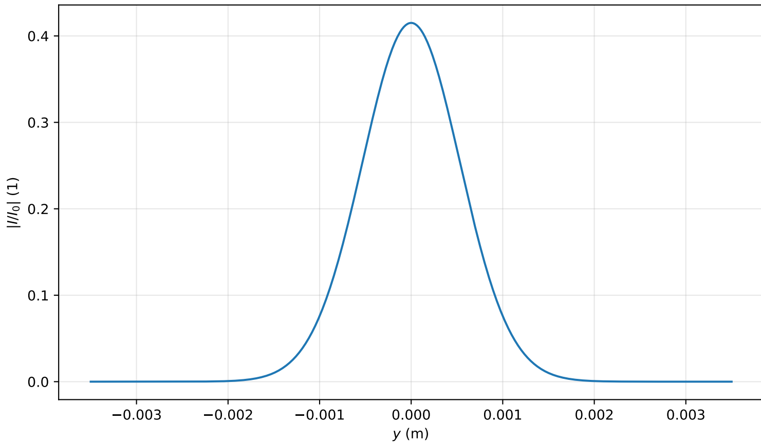
Intensity profile I(x=0, y, z=2.548)/I_0 , P_{in}=0.1P_{cr} , artificial time
